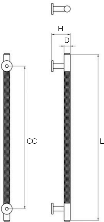
All dimensions are in mm
